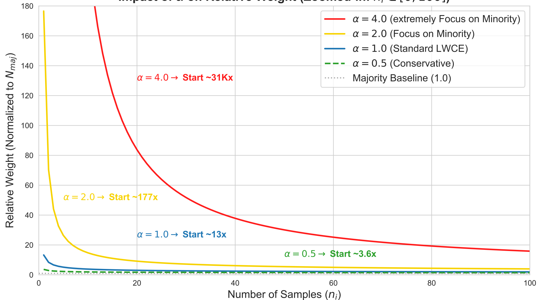
Impact of \alpha on Relative Weight (Zoomed-in: n_i \in [0, 100] )
